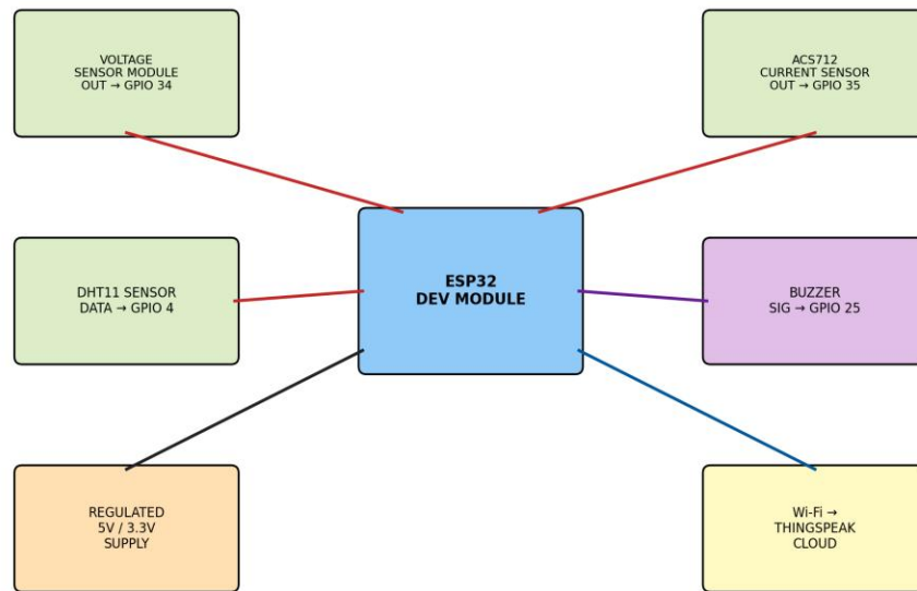
DIESEL GENERATOR MONITORING - CIRCUIT CONNECTION DIAGRAM
